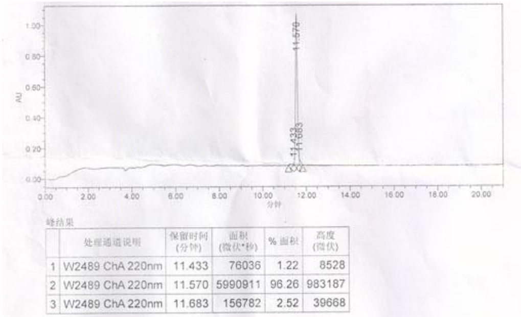
Figure 1. HPLC
