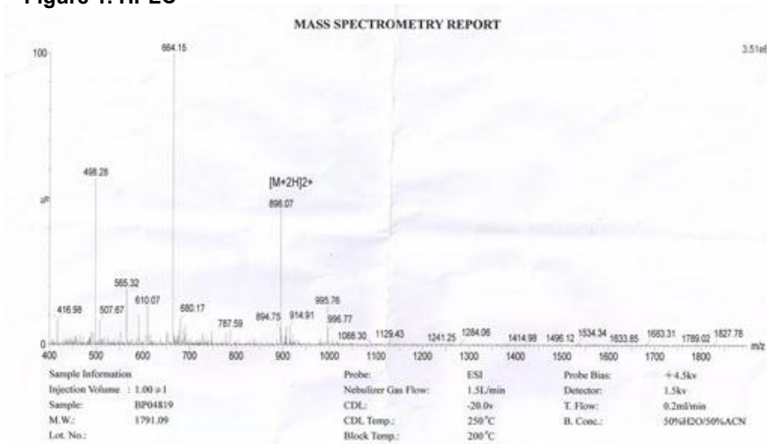
Figure 2. MASS Spectrometry
