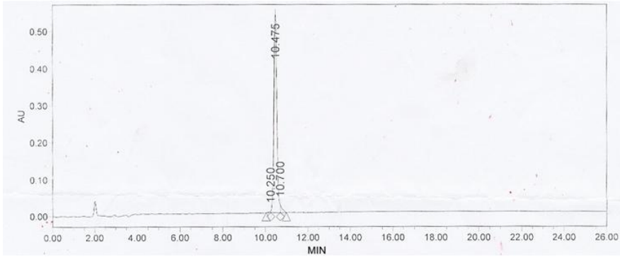
Figure 1. HPLC
