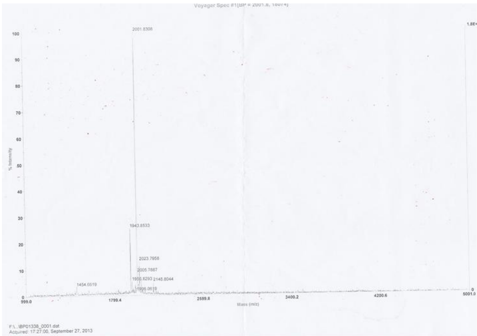
Figure 2. MASS Spectrometry
